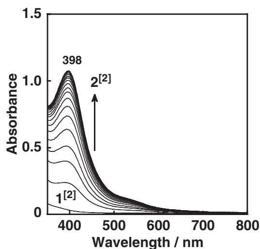
Figure 3. Spectral change observed upon addition of \text{H}_2\text{O}_2 (3.0 mM) to an acetone solution of 1 [2] (0.6 mM) in the presence of triethylamine (0.6 mM) at −70 °C generating bis( \mu -oxo)dinickel(III) complex 2 [2] .
