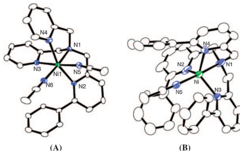
Figure 1. ORTEP drawings of the cationic parts of (A) [\text{Ni}(\text{Ph}_1\text{tpa})(\text{CH}_3\text{CN})_2](\text{ClO}_4)_2 ( 1 II ) and (B) [\text{Ni}(\text{Ph}_3\text{tpa})(\text{CH}_3\text{CN})](\text{ClO}_4)_2 ( 1 III ) showing 50% probability thermal ellipsoids. The hydrogen atoms are omitted for simplicity.
